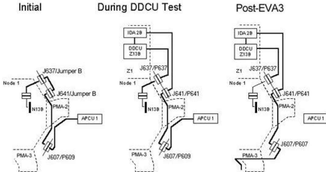
Figure 3. DDCU-HP Aliveness Test
