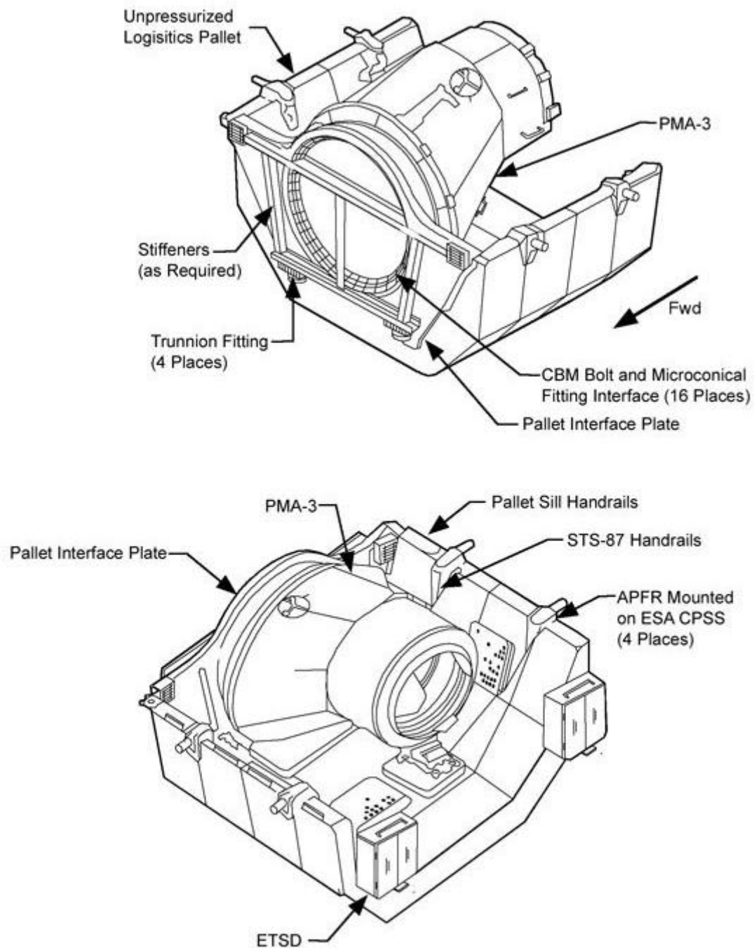
Figure 9. PMA-3 Mounted in SLP
