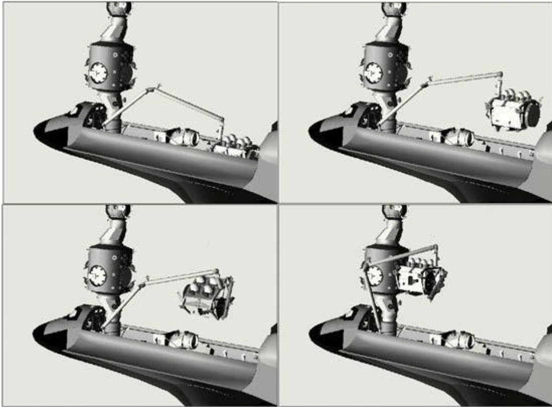
Figure 1. Z1 Installation
