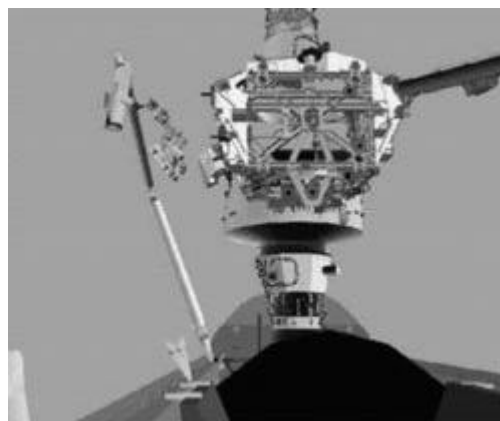
Figure 8. DDCU-HP Installation
