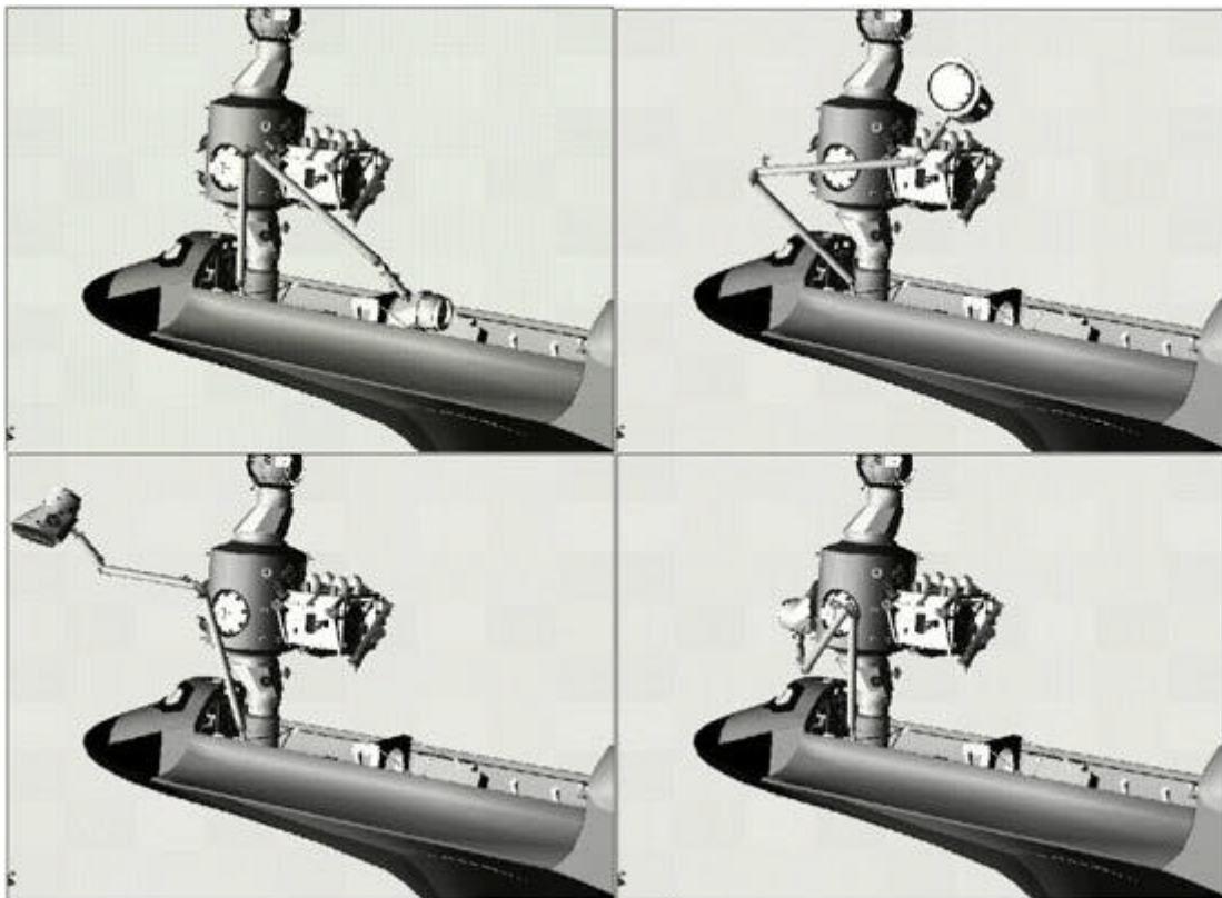
Figure 2. PMA-3 Installation
