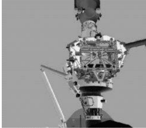
Figure 12. Connection of Final Z1 Umbilicals
